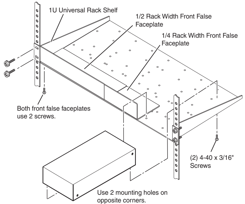
Figure 4. Rack Mounting the PS 125
