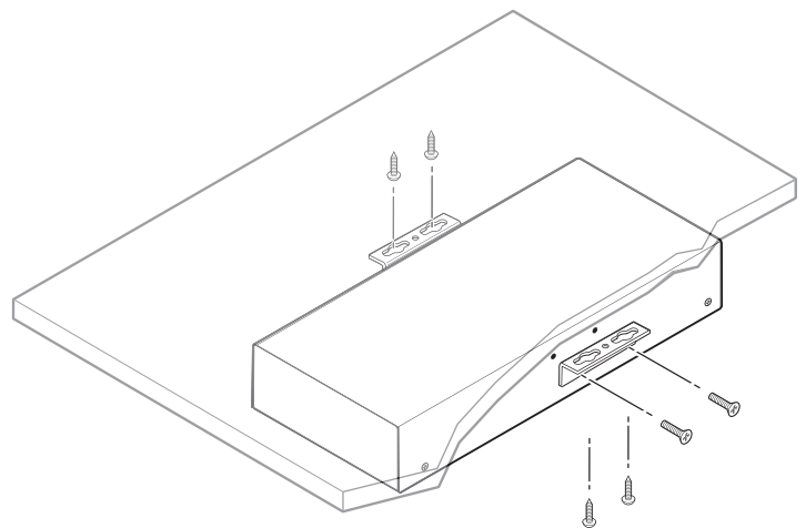
Figure 5. Under-desk Mounting the PS 125
