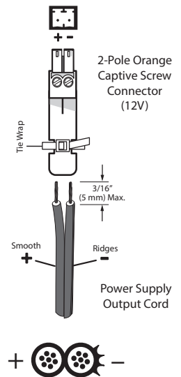
Figure 3. DC Output Wiring
