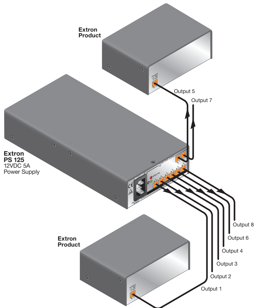
Figure 2. PS 125 Application Diagram
