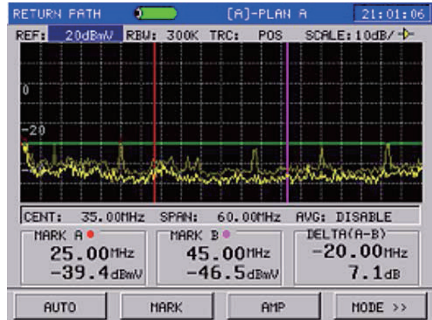
Return Path Spectrum
