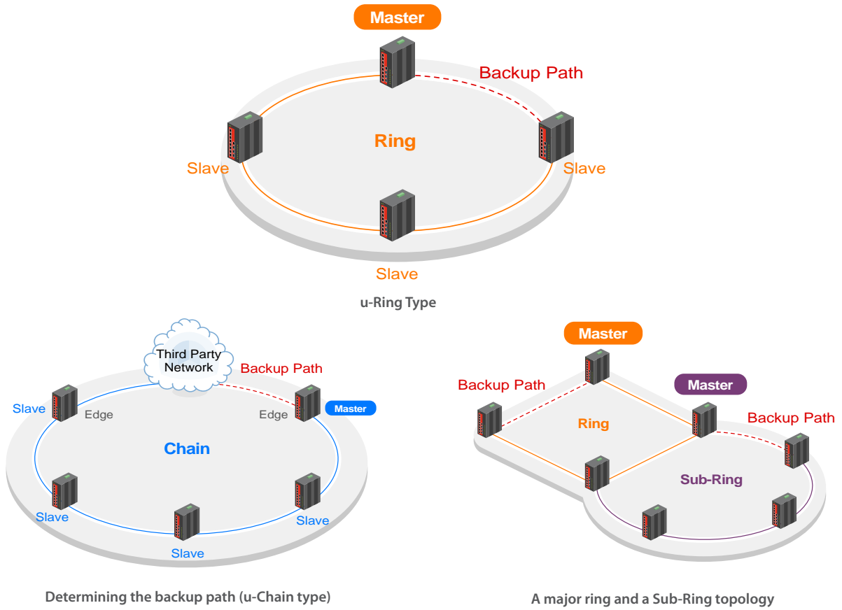
Figure 5 : u-Ring Type
