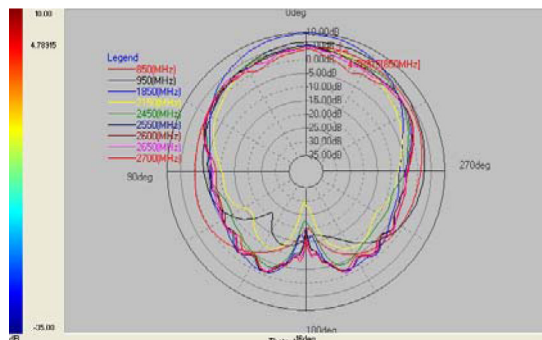
H-Plane at all frequencies
