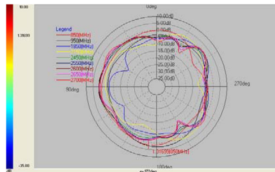
E-Plane at all frequencies
